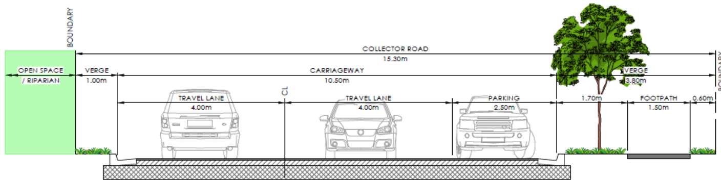
TYPICAL SECTION - COLLECTOR ROAD (ADJACENT TO BUSHFIRE HAZARD / PASSIVE DISTRICT PARK / LINEAR PARKS) (1 - 10.5 - 3.8)
