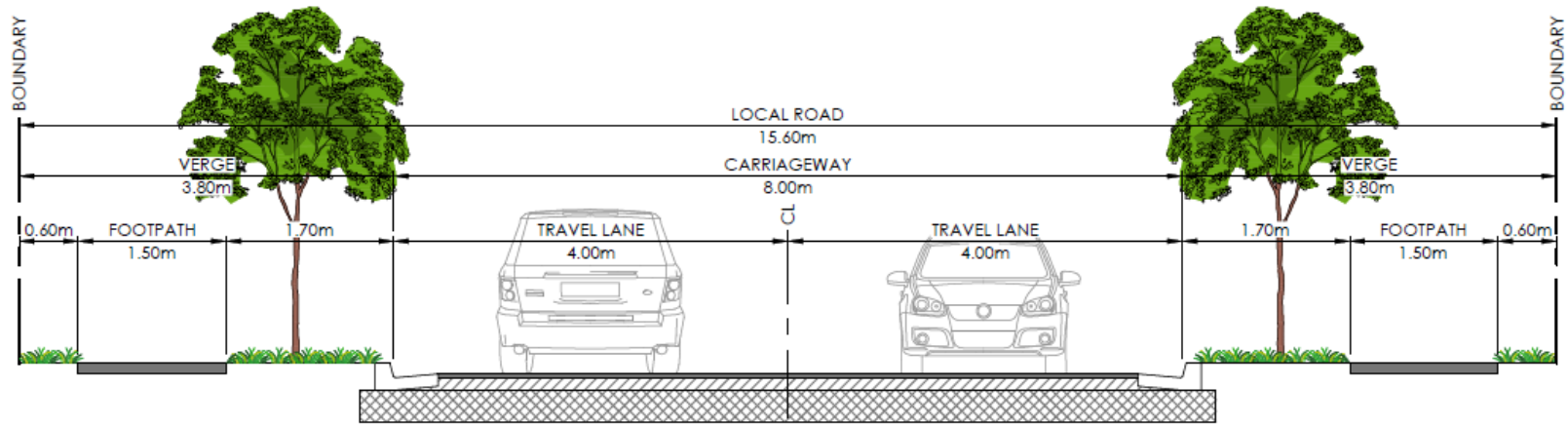
TYPICAL SECTION - MINOR LOCAL ROAD (3.8 - 8 - 3.8)
