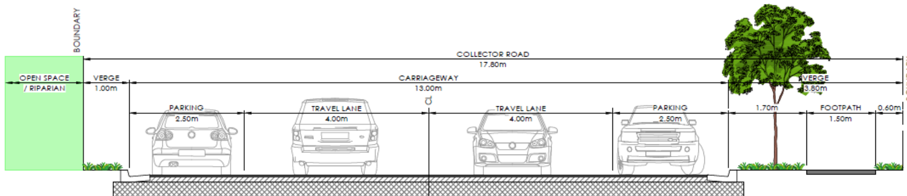
TYPICAL SECTION - COLLECTOR ROAD (ADJACENT TO BUSHFIRE HAZARD / ACTIVE DISTRICT PARK) (1 - 13 - 3.8)
